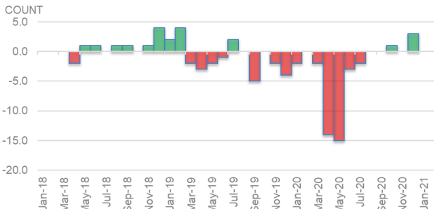
Niobrara Region Month-On-Month Rig Count
