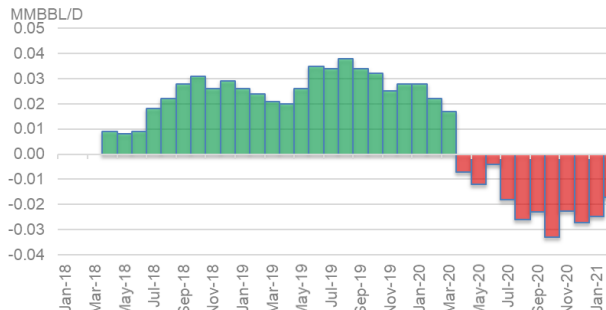
Appalachia Region Month-On-Month Oil Production
