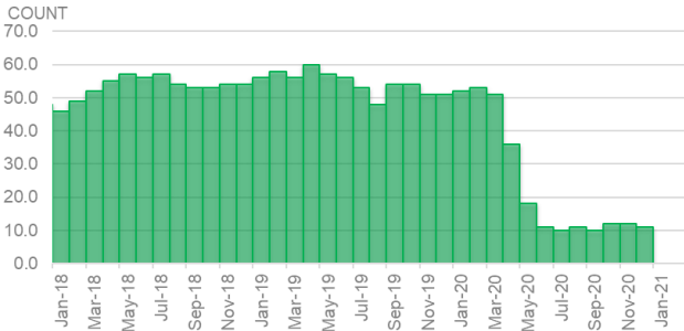
Bakken Region Year-On-Year Rig Count
