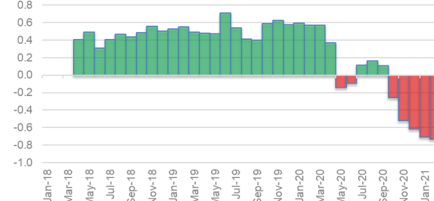
Niobrara Region Month-On-Month Natural Gas Production
