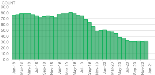
Appalachia Region Year-On-Year Rig Count
