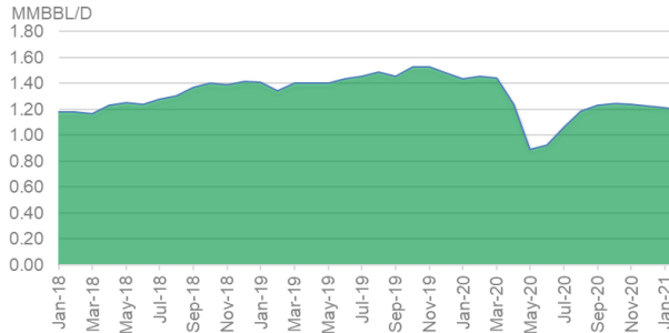
Bakken Region Year-On-Year Oil Production
