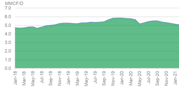
Niobrara Region Year-On-Year Natural Gas Production
