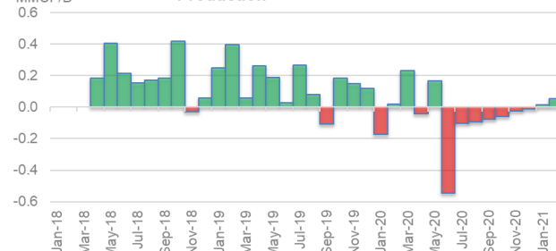
Haynesville Region Month-On-Month Natural Gas Production
