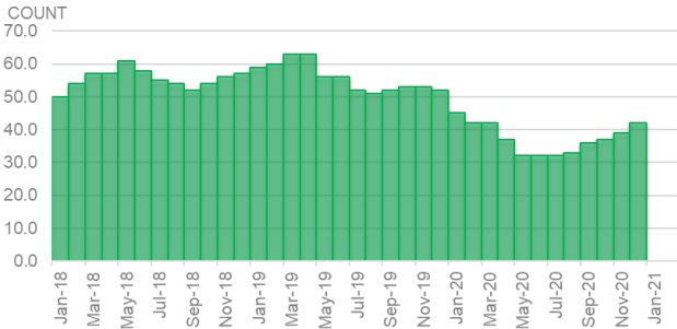
Haynesville Region Year-On-Year Rig Count
