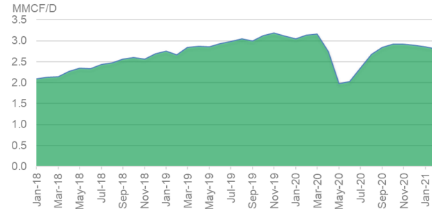
Bakken Region Year-On-Year Natural Gas Production
