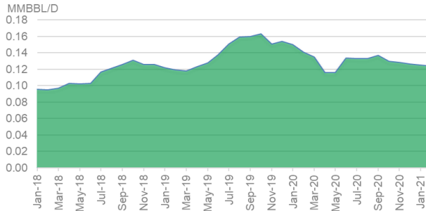
Appalachia Region Year-On-Year Oil Production
