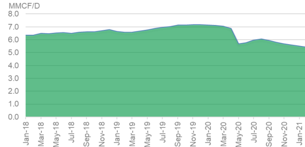
Eagle Ford Region Year-On-Year Natural Gas Production
