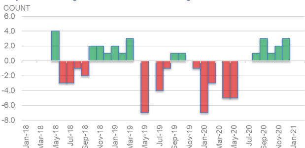
Haynesville Region Month-On-Month Rig Count
