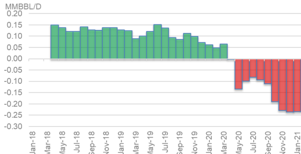
Niobrara Region Month-On-Month Oil Production
