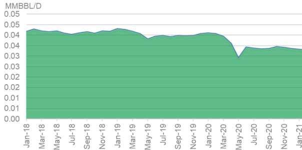
Haynesville Region Year-On-Year Oil Production
