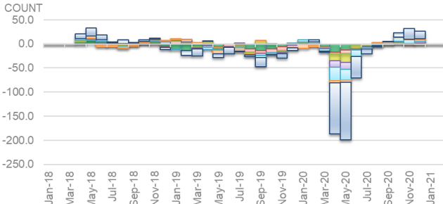
Rig Count MoM Growth
