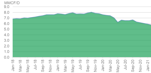
Anadarko Region Year-On-Year Natural Gas Production
